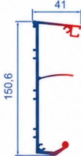
T.2520 2,394 KG/MT Duvar Dayama Profili
