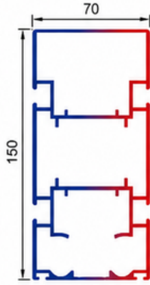
T.2701 - 3,883 KG/MT
